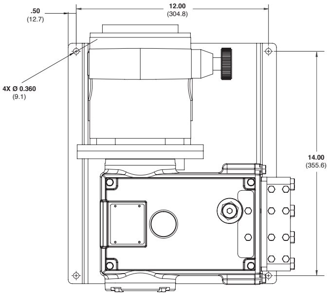
Metallic Heads with Manual Adjustment
